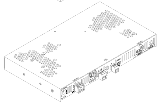
DXF-RX-SMS (Isometric Views)
