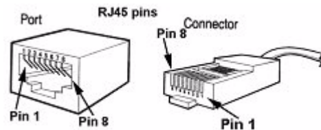
FIG. 44 RJ-45 Pinouts
