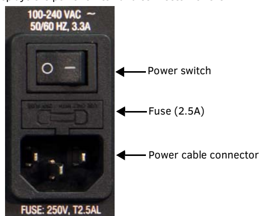
FIG. 63 Power Connector/Switch/Fuse
